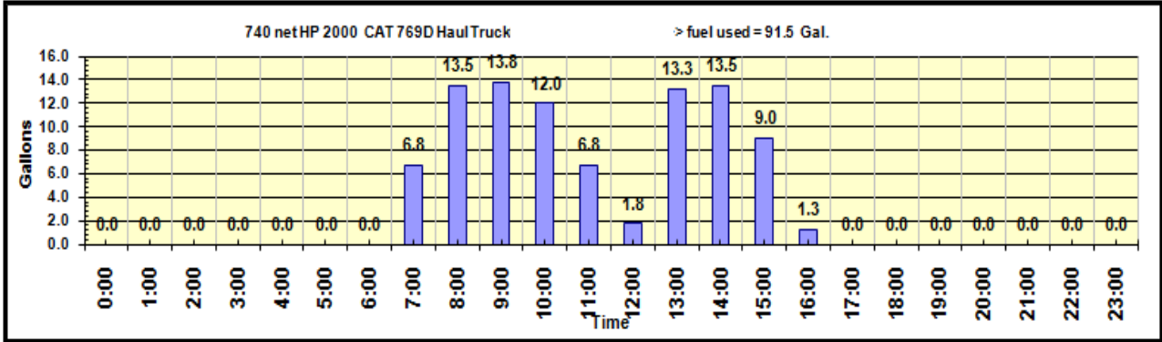
Fuel Use in Gallons per Hour.
